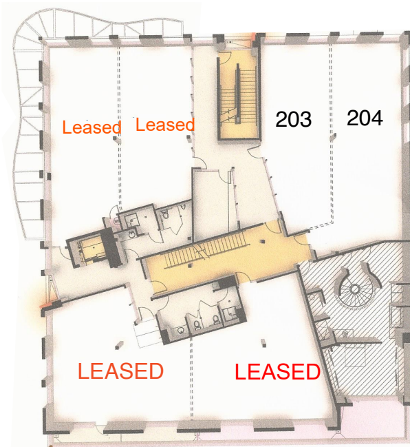
SECOND FLOOR PLAN 0 8' 16' 32' SCALE: 1"=16' ■ PRIMARY CIRCULATION ■ SERVICE AREAS ■ SHARED SPACE ■ LEASABLE SPACE ■ CURRENTLY LEASED - - - GLASS CEILING
